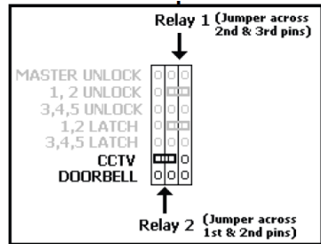
■ CCTV/Doorbell Setup
