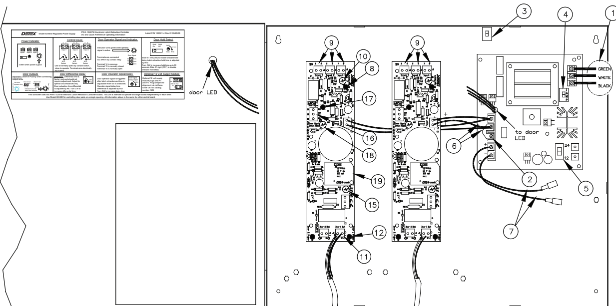
Connections for 2nd bank of doors
