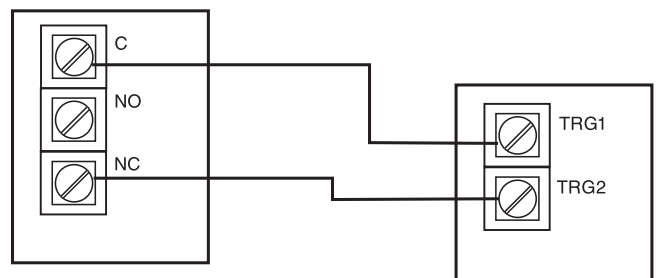
Fig. 6 - Multiple AL175UL(X) power supply connections:
